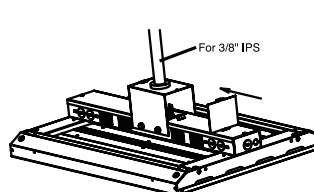
Stem Mount
